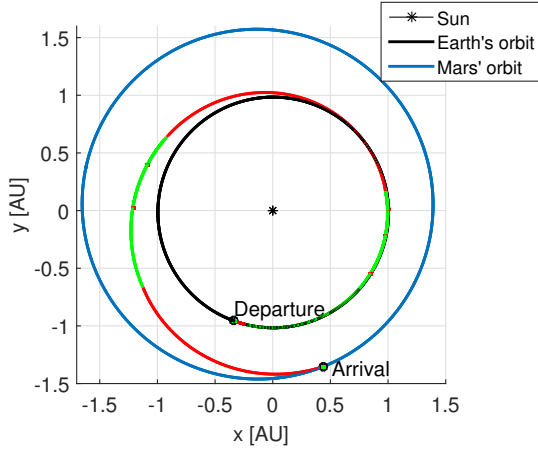
Figure 4: Earth-Mars. IMAgIne's interplanetary low-thrust outbound trajectory to Mars.
