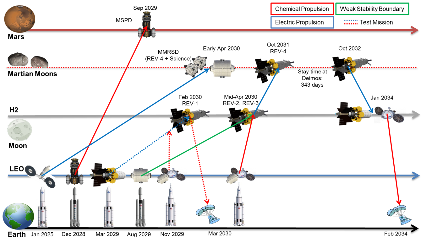
Figure 1: IMAgInE's mission architecture.
